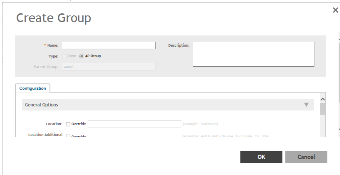
FIGURE 47 Create Groups
